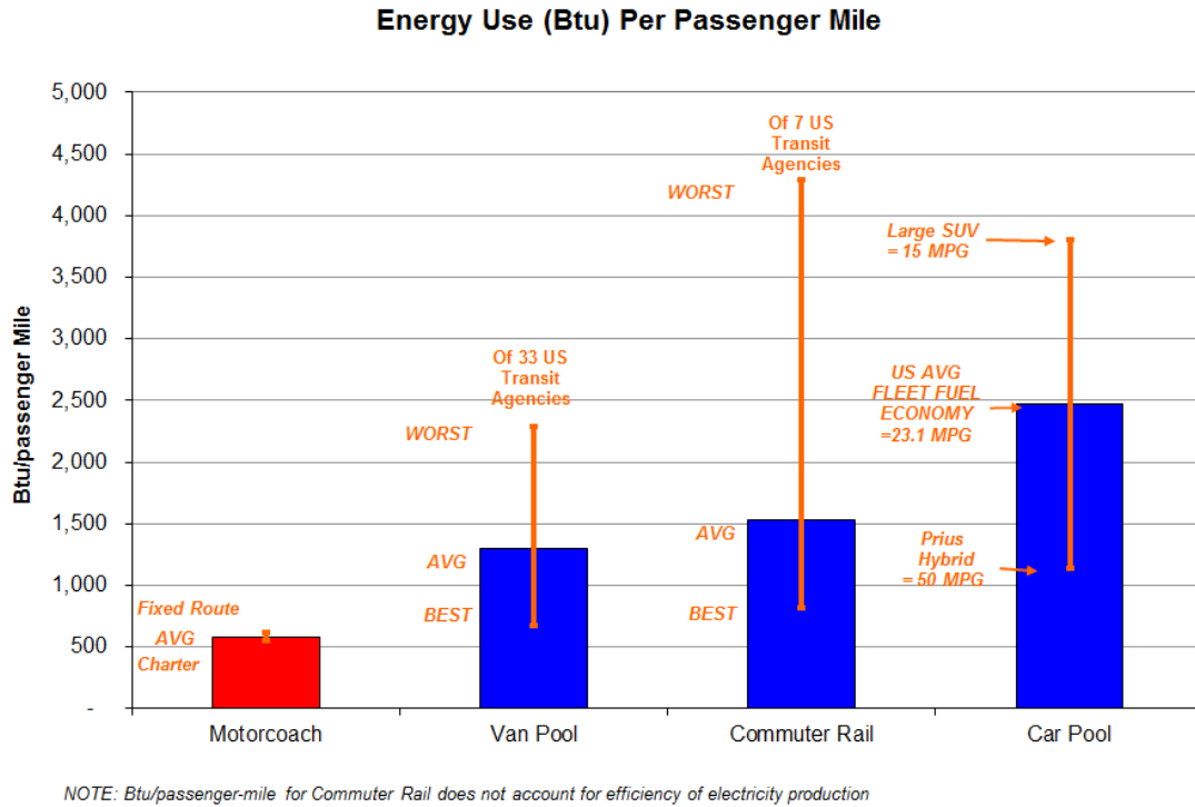
Figure 1.4 Range of Energy Use (btu) per Passenger-Mile, Selected Modes
